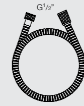
C28300 Metal hose Double fastened brass shower hose 1/2" by 1/2", 1.5m length
